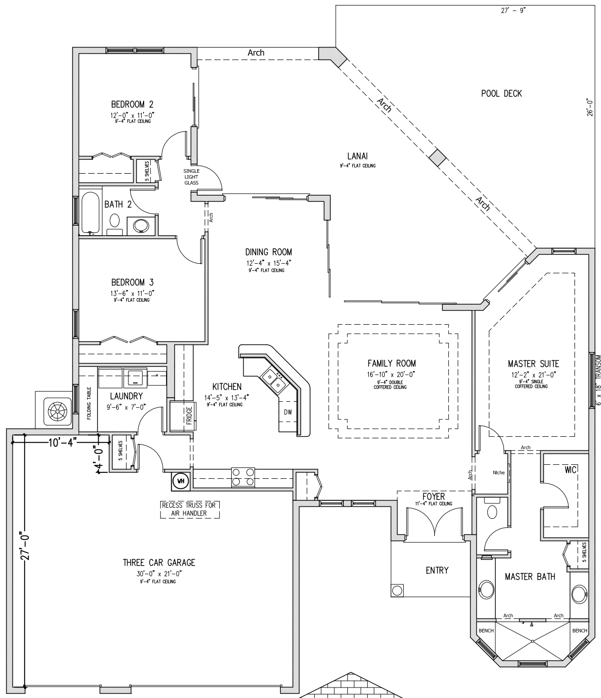
FLOOR PLAN
