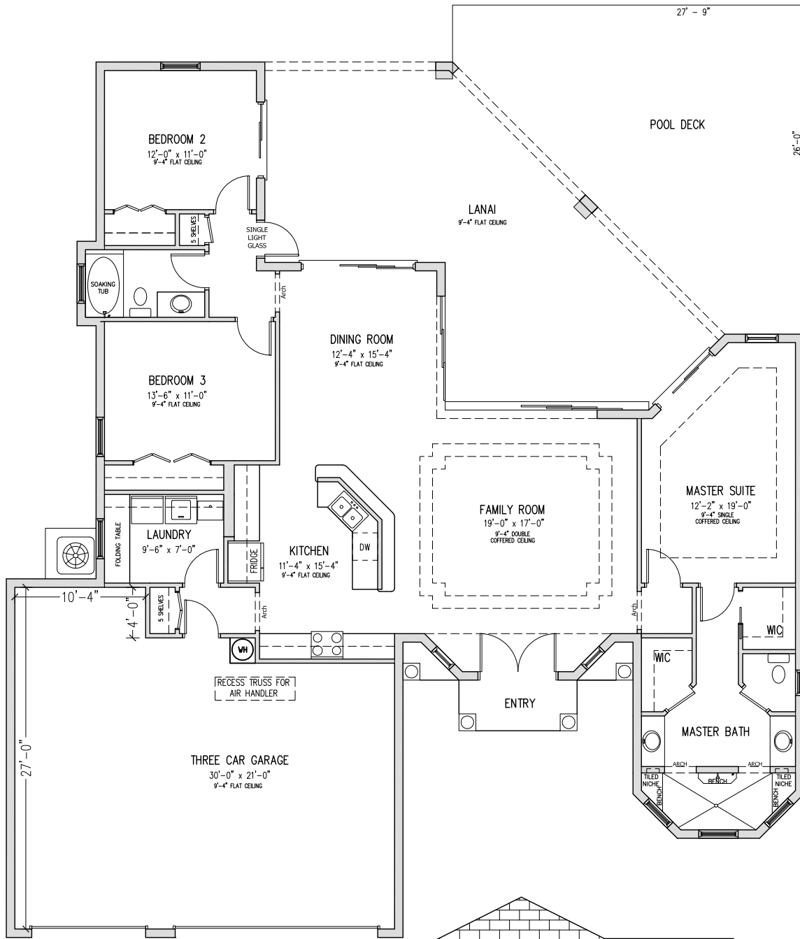
FLOOR PLAN
